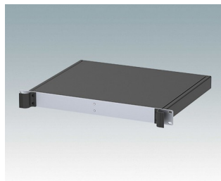
M6219159 COMBIMET 19" 1Ux365mm Aluminium Noir RAL 9005 43,6x482,6x365mm
