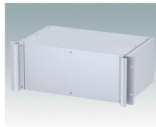
M6219435 COMBIMET 19" 4Ux265mm Aluminium Gris clair RAL 7035 177x482,6x265mm
